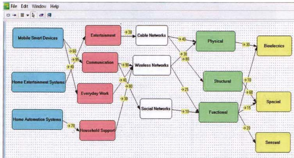
Fig. 2 A screen shot from I-SCIP-MA environment model for smart homes cyber threats identification.
